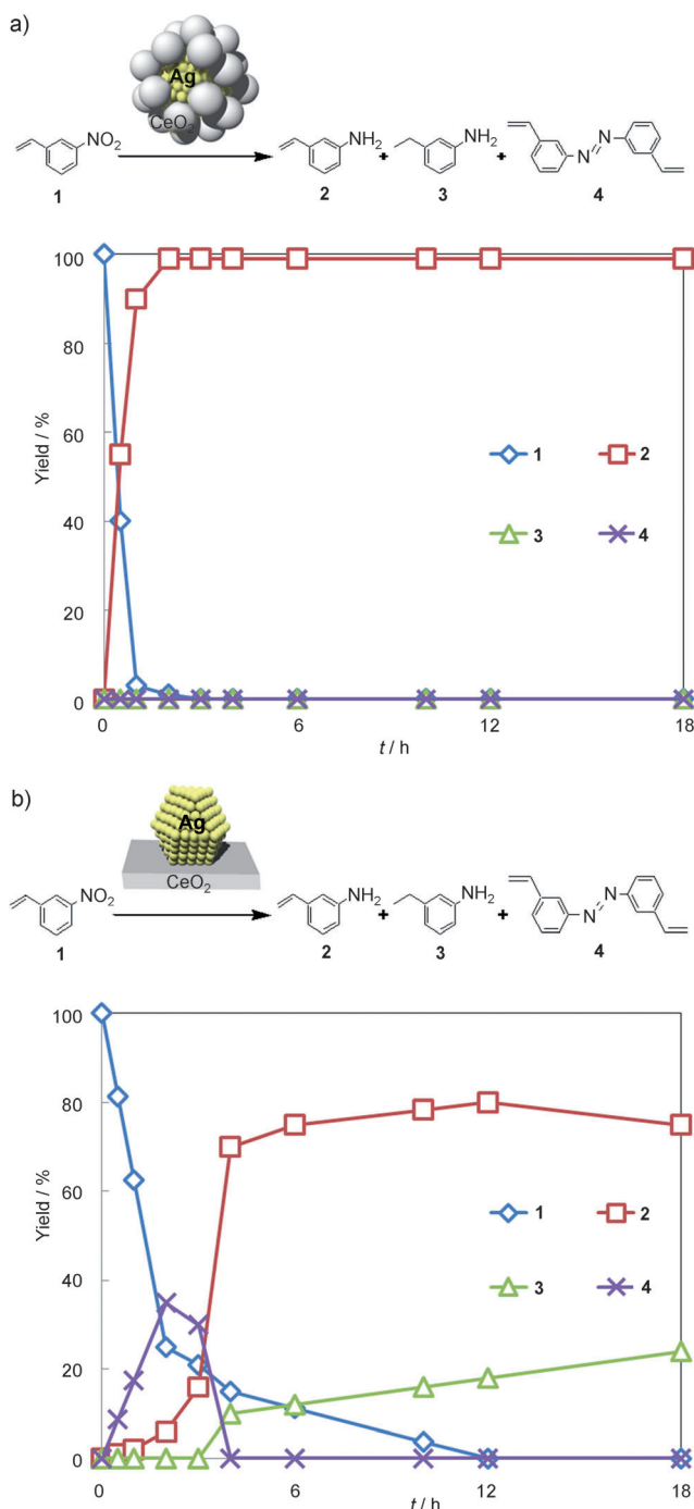
Figure 4. Time course of the reduction of 1 with H 2 using a) AgNPs@-CeO 2 and b) AgNPs/CeO 2 .
